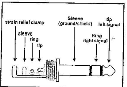
1/4 inch TRS headphones connector
