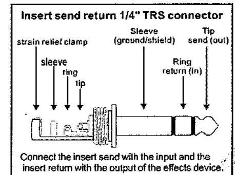
Insert send/return stereo plug
