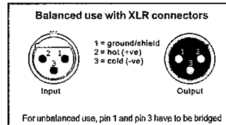
XLR connections
