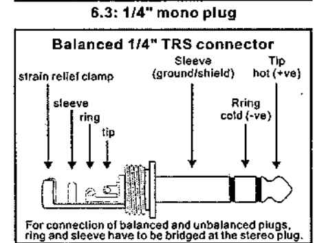
Balanced 1/4 inch TRS connector
