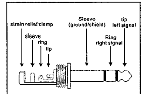
1/4 inch TRS headphones connector
